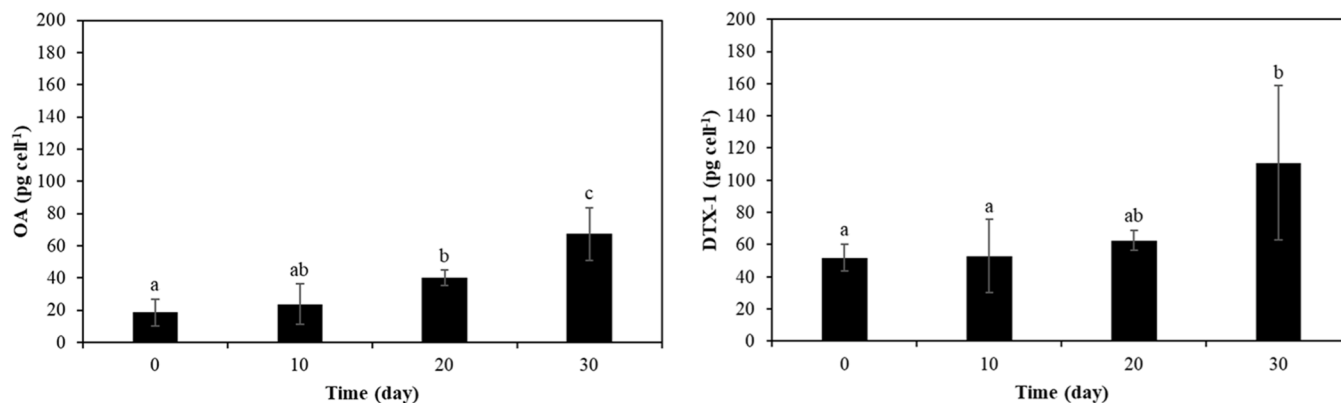
Fig. 5. Toxins (OA and DTX-1) contents in Prorocentrum lima ( pg\ cell^{-1} ) measured on 0, 10, 20 and 30 day after nutrient supply stopped. Each coordinate is the overall mean with standard deviation of 5 replicates. Different letters on the graph mean significant differences from others ( p < 0.05 ).
